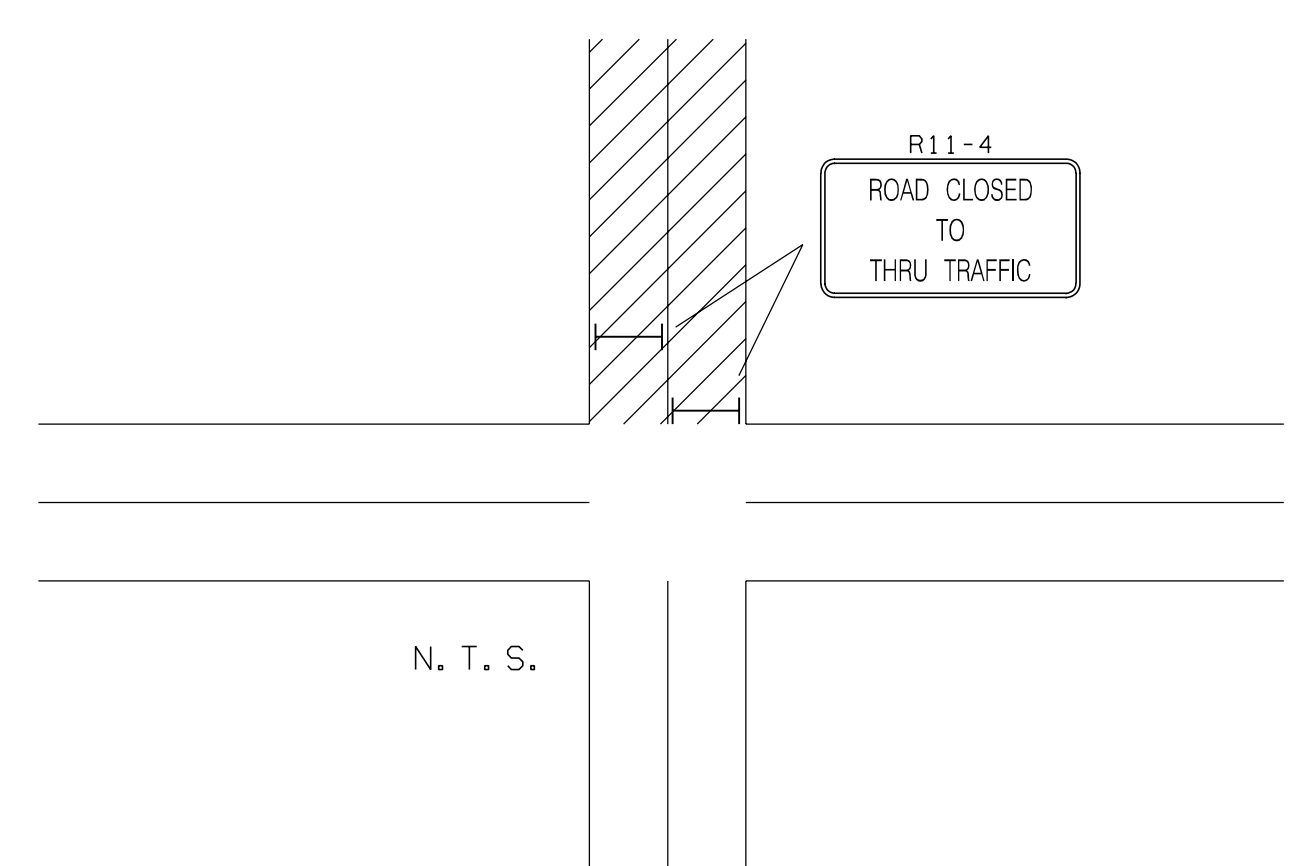
ADDITIONAL DEVICES REQUIRED WHEN ROAD CLOSED DIRECTLY AT INTERSECTION
