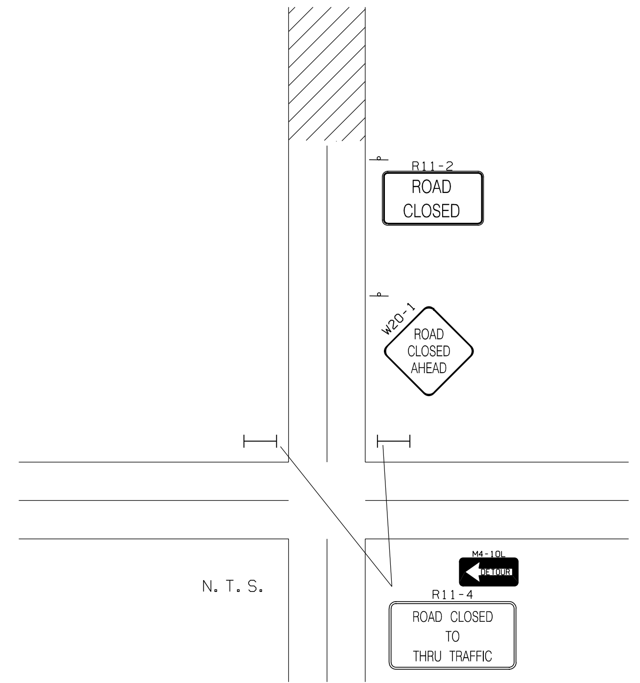
ADDITIONAL DEVICES REQUIRED WHEN ROAD CLOSED AWAY FROM INTERSECTION
